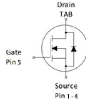
Schematic Diagram
