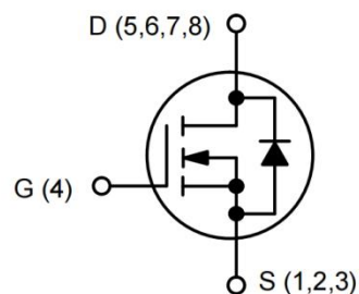
Schematic Diagram
