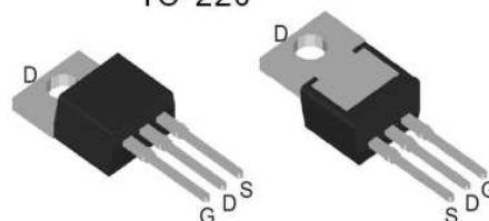
TO-220
